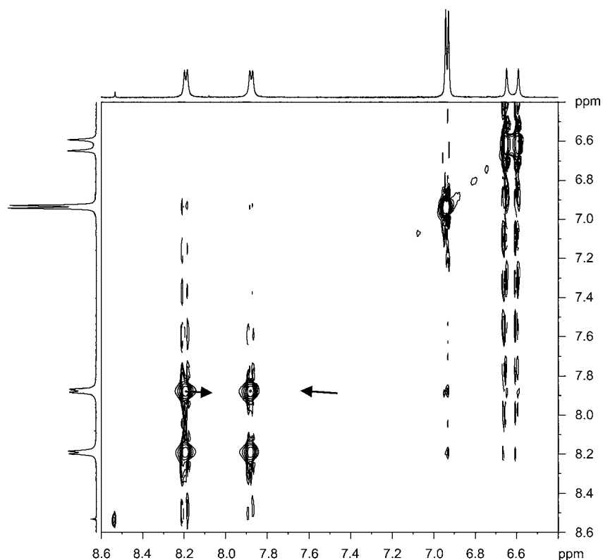
Fig. 3. The lower-field section of NOESY spectrum of 4 . The arrows indicate the exchanged cross-peaks between H–C(2') and H–C(6) of 4a and 4b .
