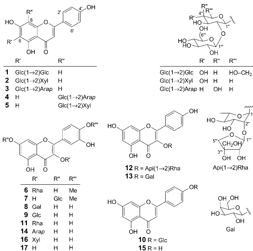
Fig. 1. Structures of compounds 1–17
