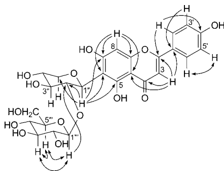
Fig. 2. Key HMBCs and NOESY correlations of compound 2 ( \text{CD}_3\text{OD} , 600 MHz)
